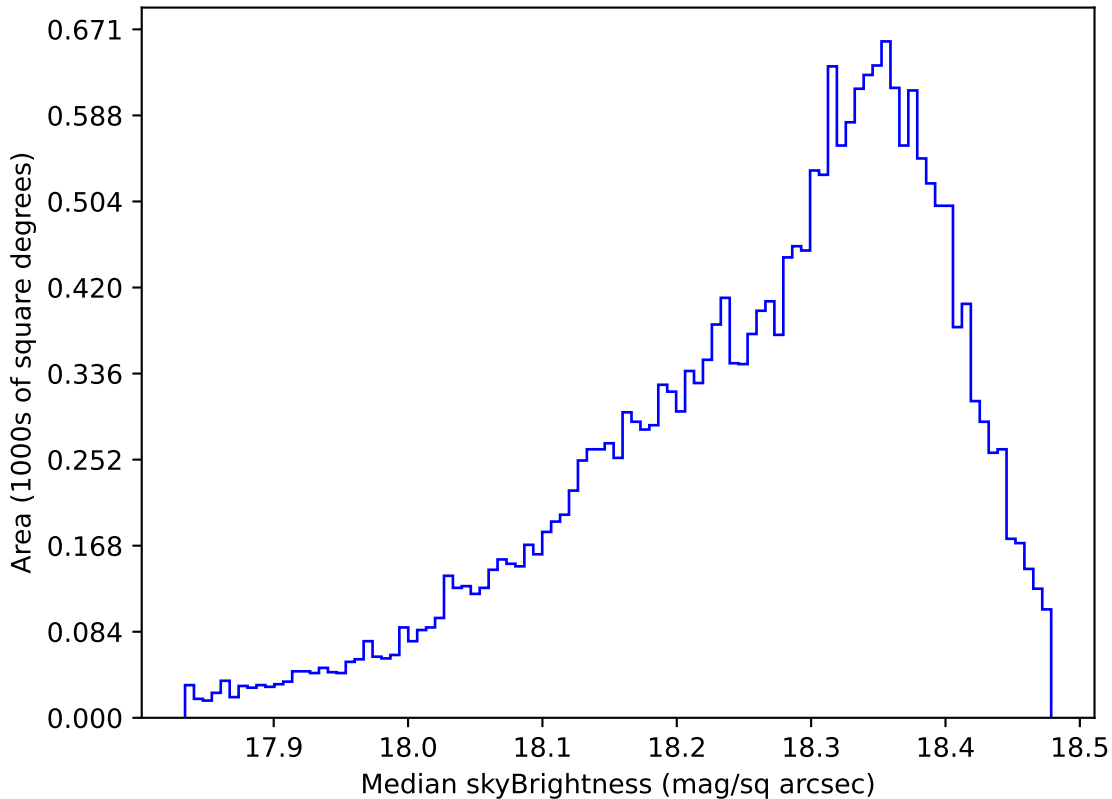
too_elab_r32_d3_giz_v3.4_10yrs Yr 1 y band: Median skyBrightness
