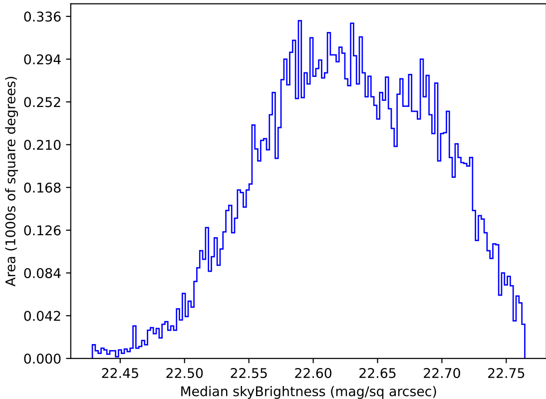
too_elab_r32_d3_giz_v3.4_10yrs Yr 1 u band: Median skyBrightness
