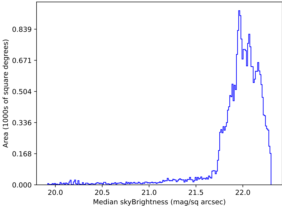
too_elab_r32_d3_giz_v3.4_10yrs Yr 1 g band: Median skyBrightness
