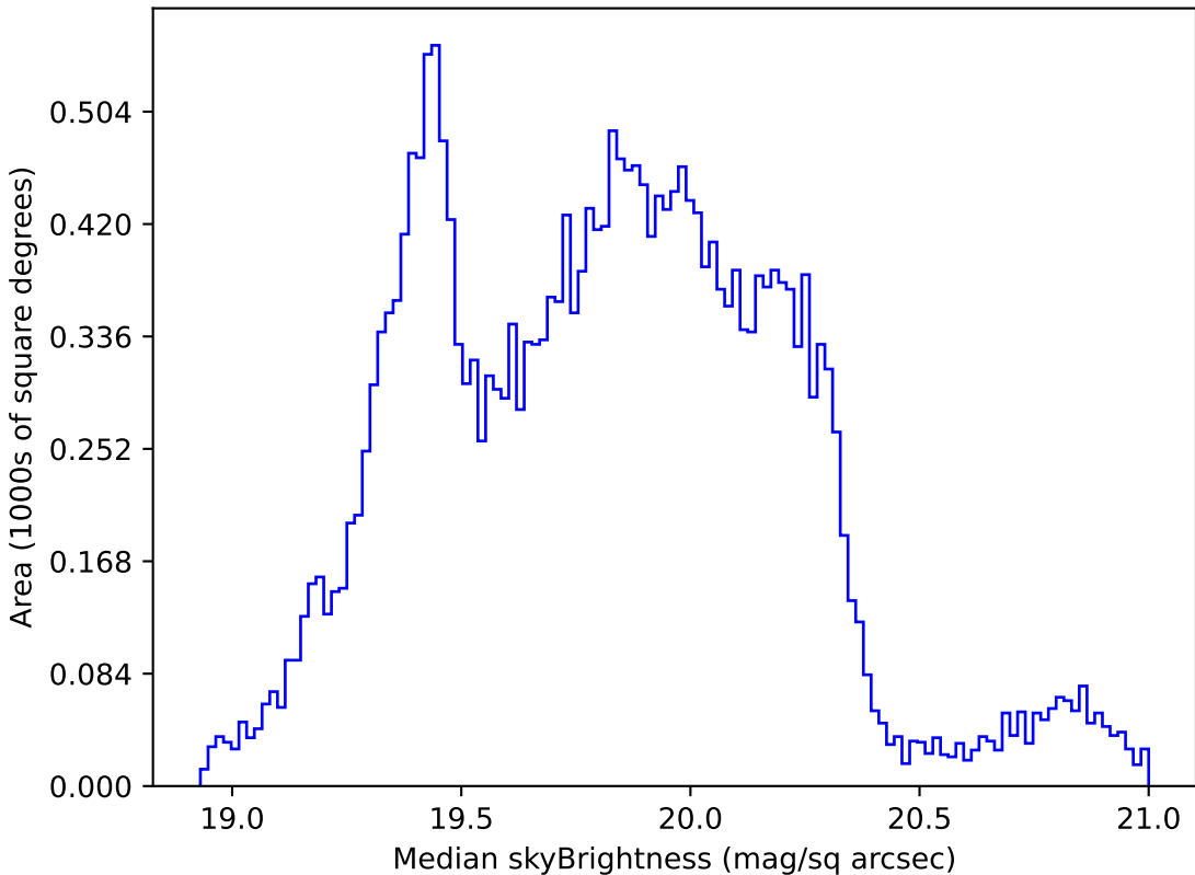
too_elab_r32_d3_giz_v3.4_10yrs Yr 1 all bands: Median skyBrightness
