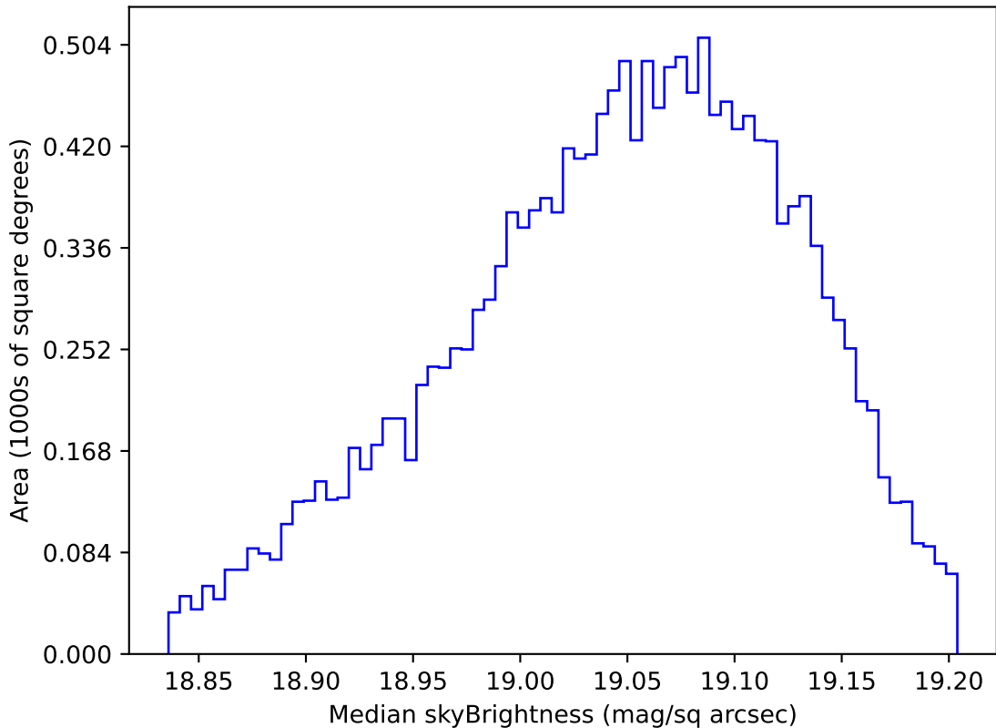
too_elab_r32_d3_giz_v3.4_10yrs WFD z band: Median skyBrightness
