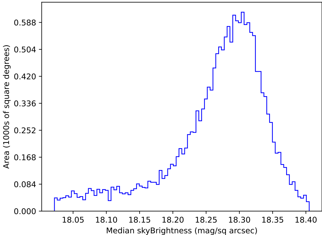
too_elab_r32_d3_giz_v3.4_10yrs WFD y band: Median skyBrightness
