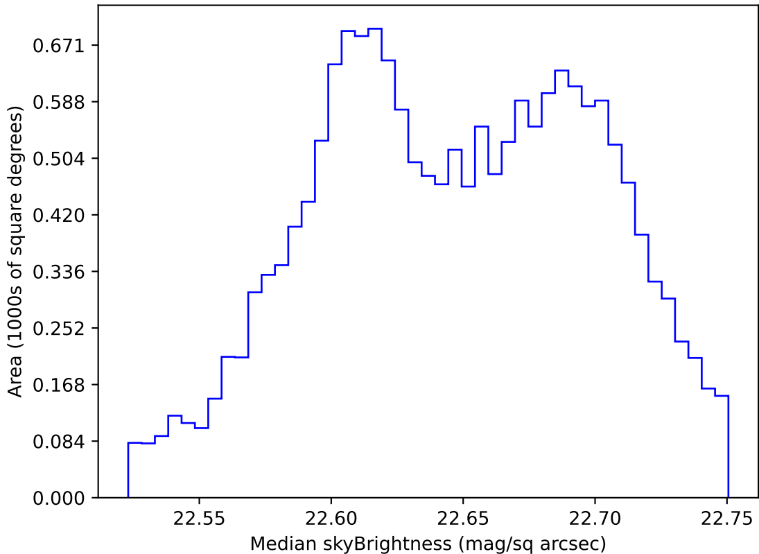
too_elab_r32_d3_giz_v3.4_10yrs WFD u band: Median skyBrightness
