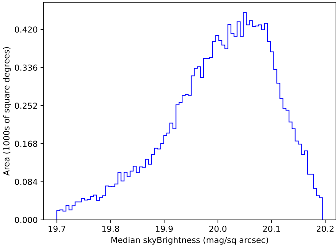
too_elab_r32_d3_giz_v3.4_10yrs WFD i band: Median skyBrightness
