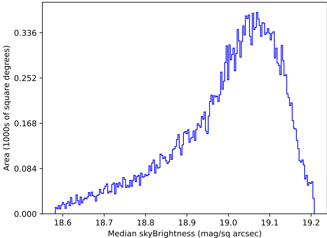
too_elab_r32_d3_giz_v3.4_10yrs All sky z band: Median skyBrightness
