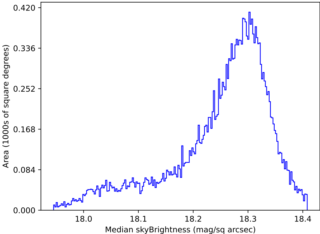
too_elab_r32_d3_giz_v3.4_10yrs All sky y band: Median skyBrightness
