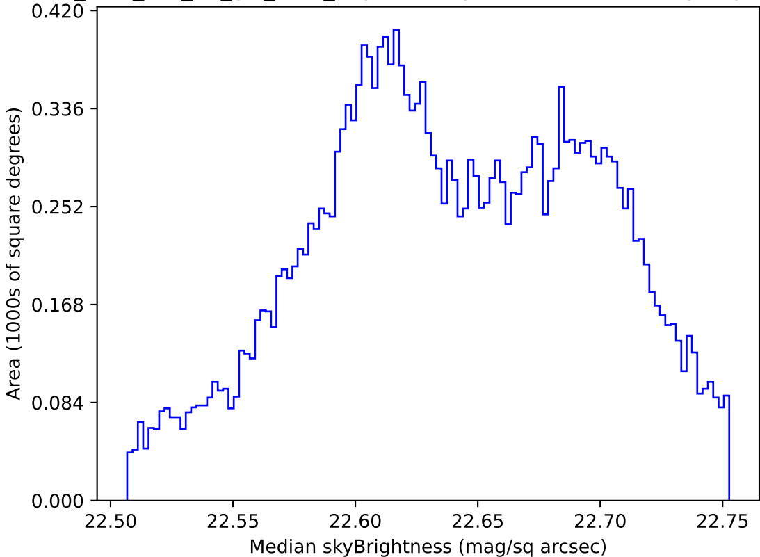
too_elab_r32_d3_giz_v3.4_10yrs All sky u band: Median skyBrightness
