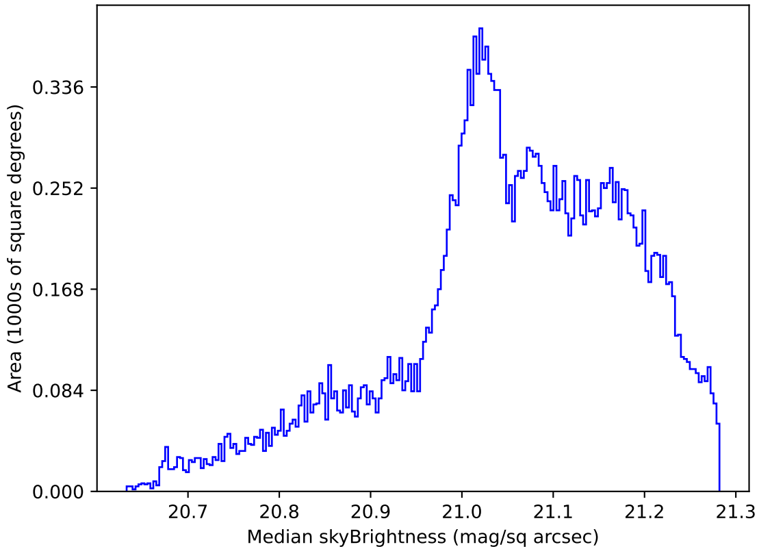
too_elab_r32_d3_giz_v3.4_10yrs All sky r band: Median skyBrightness
