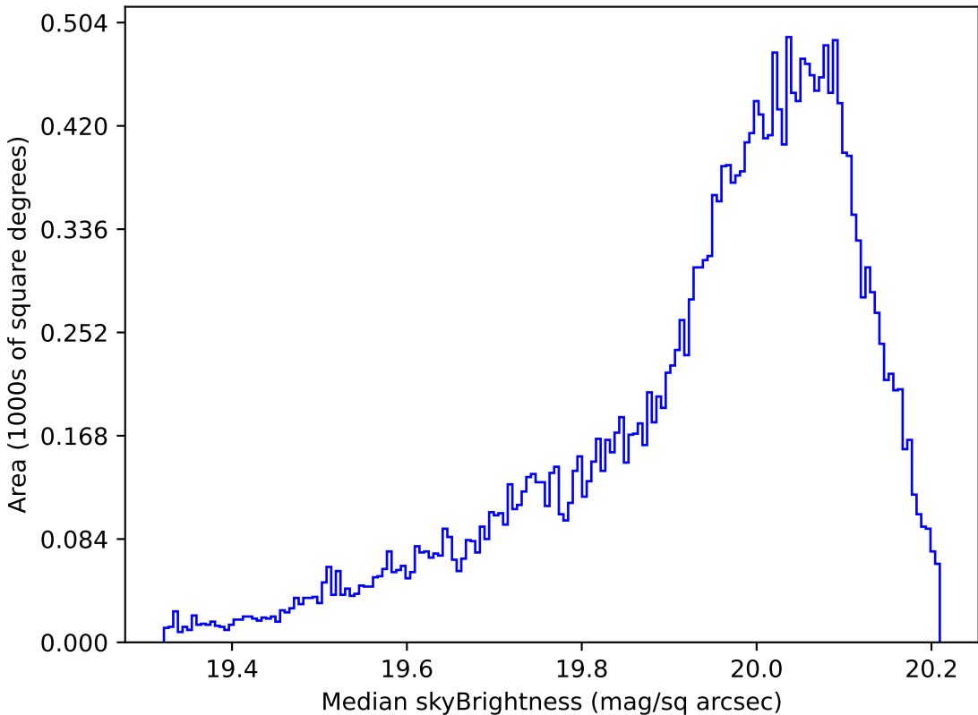
too_elab_r32_d3_giz_v3.4_10yrs All sky i band: Median skyBrightness
