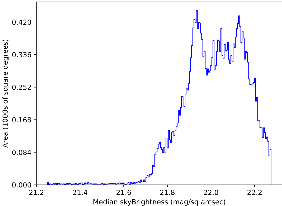
too_elab_r32_d3_giz_v3.4_10yrs All sky g band: Median skyBrightness
