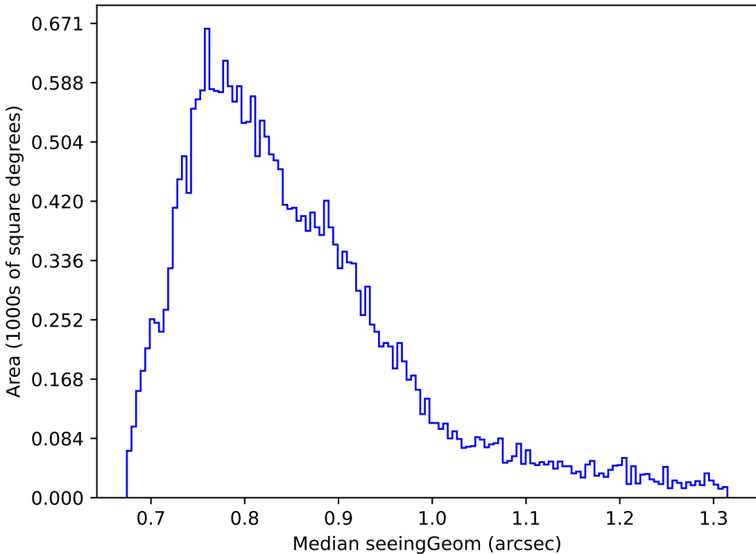
too_elab_r32_d3_giz_v3.4_10yrs Yr 1 z band: Median seeingGeom
