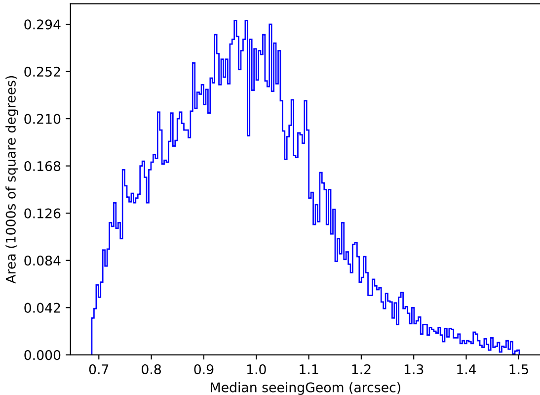
too_elab_r32_d3_giz_v3.4_10yrs Yr 1 u band: Median seeingGeom
