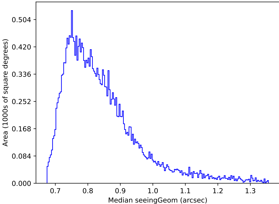
too_elab_r32_d3_giz_v3.4_10yrs Yr 1 i band: Median seeingGeom
