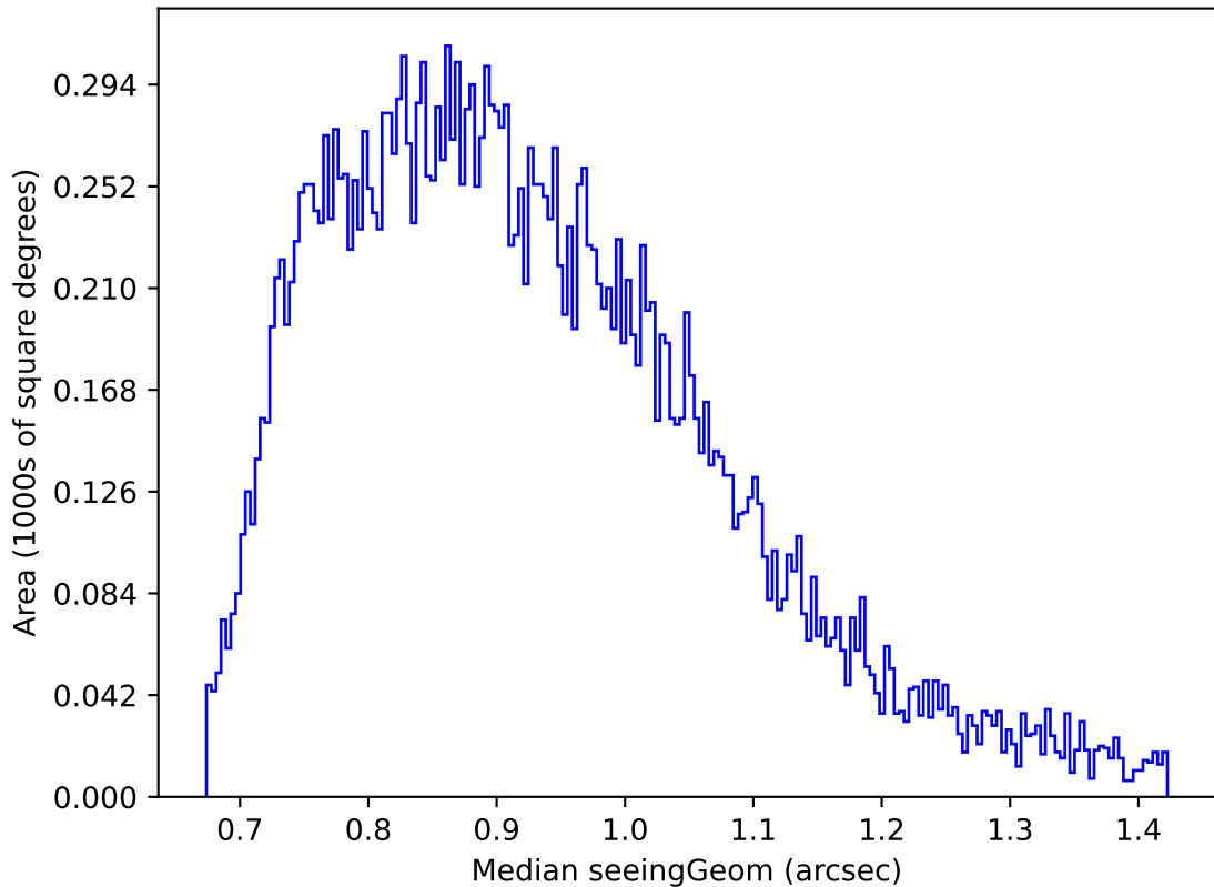
too_elab_r32_d3_giz_v3.4_10yrs Yr 1 g band: Median seeingGeom
