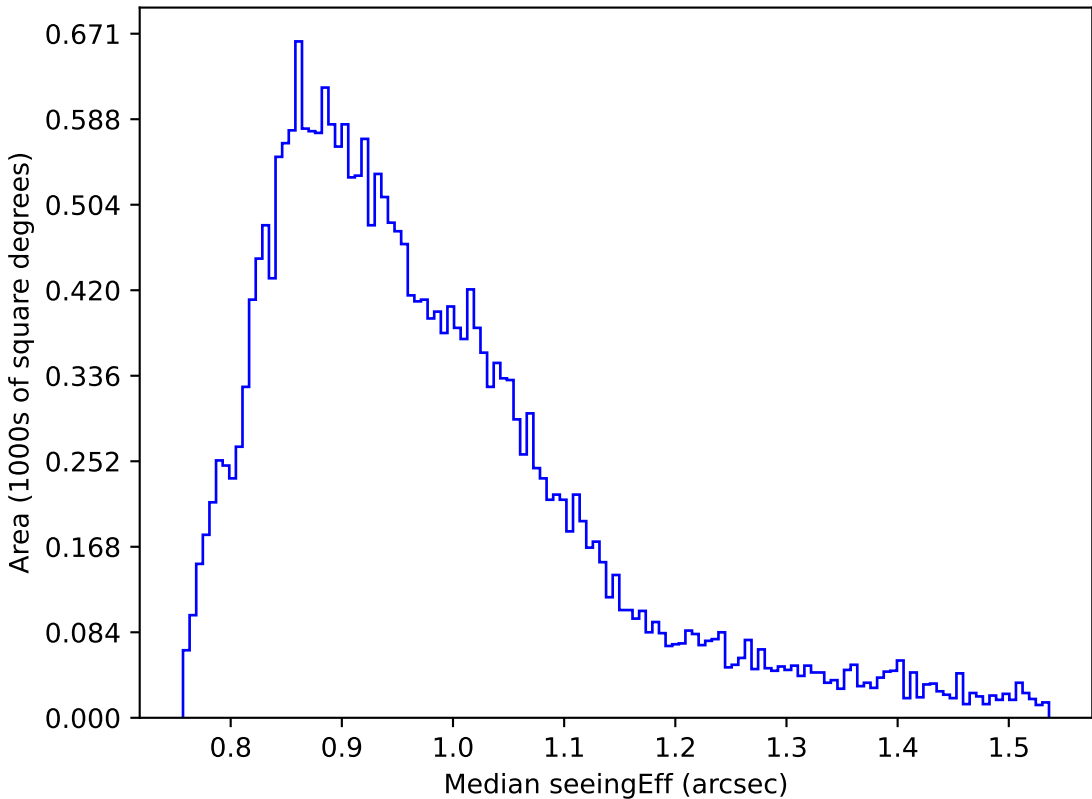
too_elab_r32_d3_giz_v3.4_10yrs Yr 1 z band: Median seeingEff
