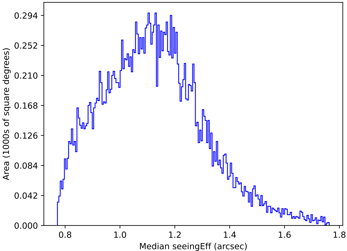
too_elab_r32_d3_giz_v3.4_10yrs Yr 1 u band: Median seeingEff
