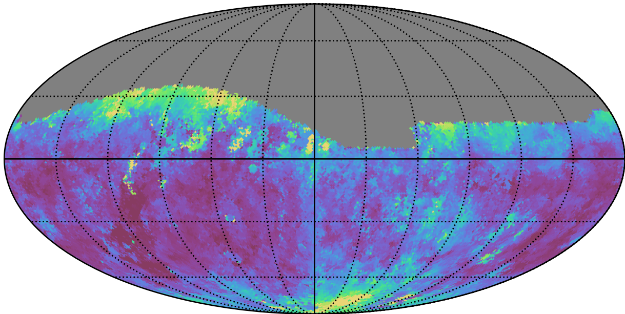
too_elab_r32_d3_giz_v3.4_10yrs Yr 1 r band: Median seeingEff
