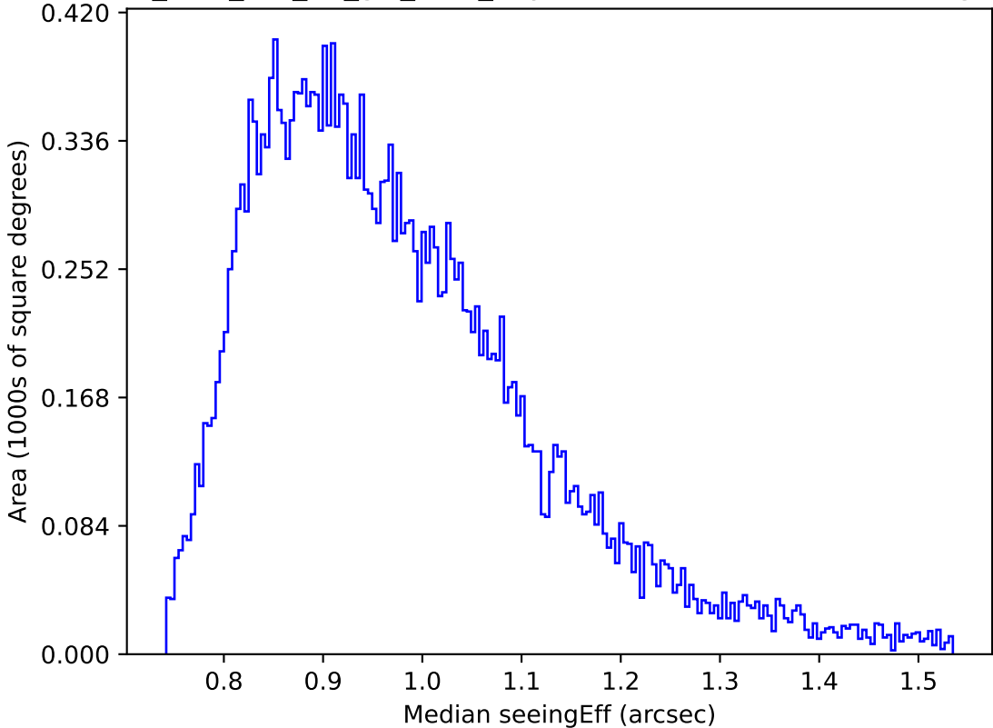
too_elab_r32_d3_giz_v3.4_10yrs Yr 1 r band: Median seeingEff
