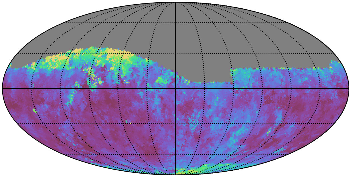
too_elab_r32_d3_giz_v3.4_10yrs Yr 1 i band: Median seeingEff
