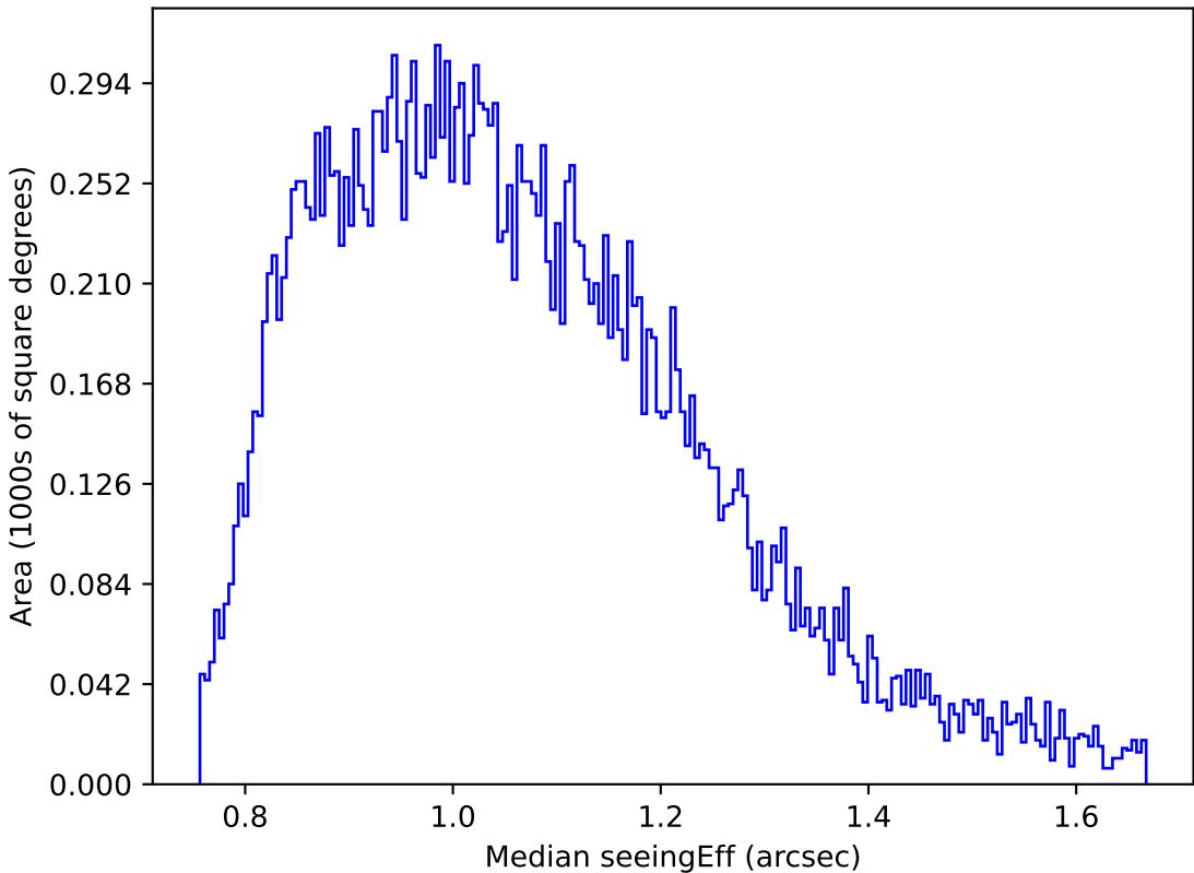
too_elab_r32_d3_giz_v3.4_10yrs Yr 1 g band: Median seeingEff
