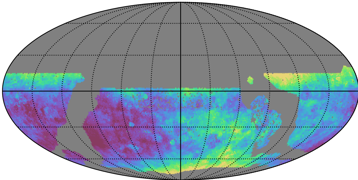
too_elab_r32_d3_giz_v3.4_10yrs WFD z band: Median seeingEff
