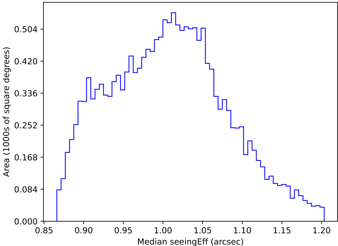
too_elab_r32_d3_giz_v3.4_10yrs WFD z band: Median seeingEff
