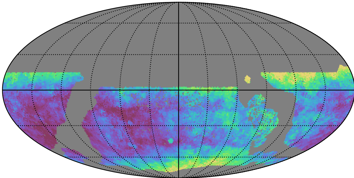
too_elab_r32_d3_giz_v3.4_10yrs WFD y band: Median seeingEff
