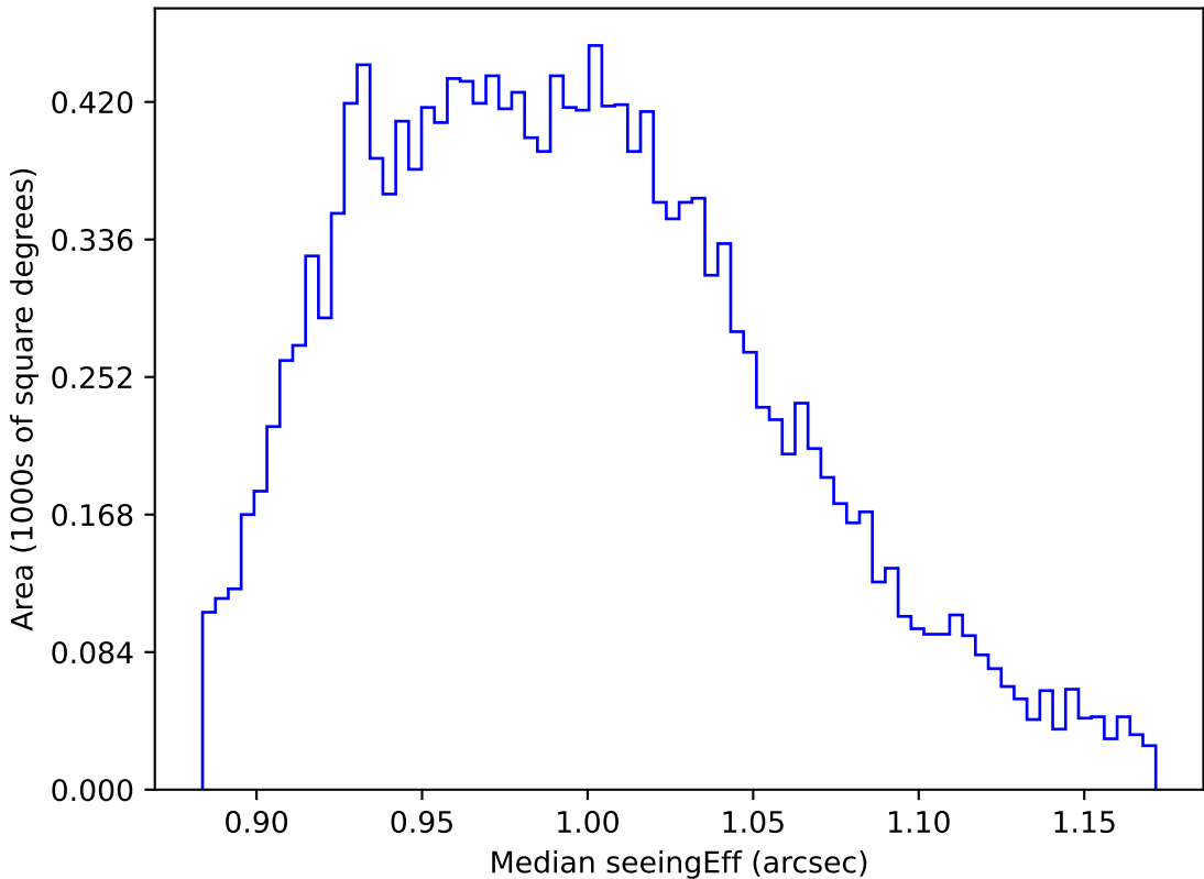
too_elab_r32_d3_giz_v3.4_10yrs WFD y band: Median seeingEff
