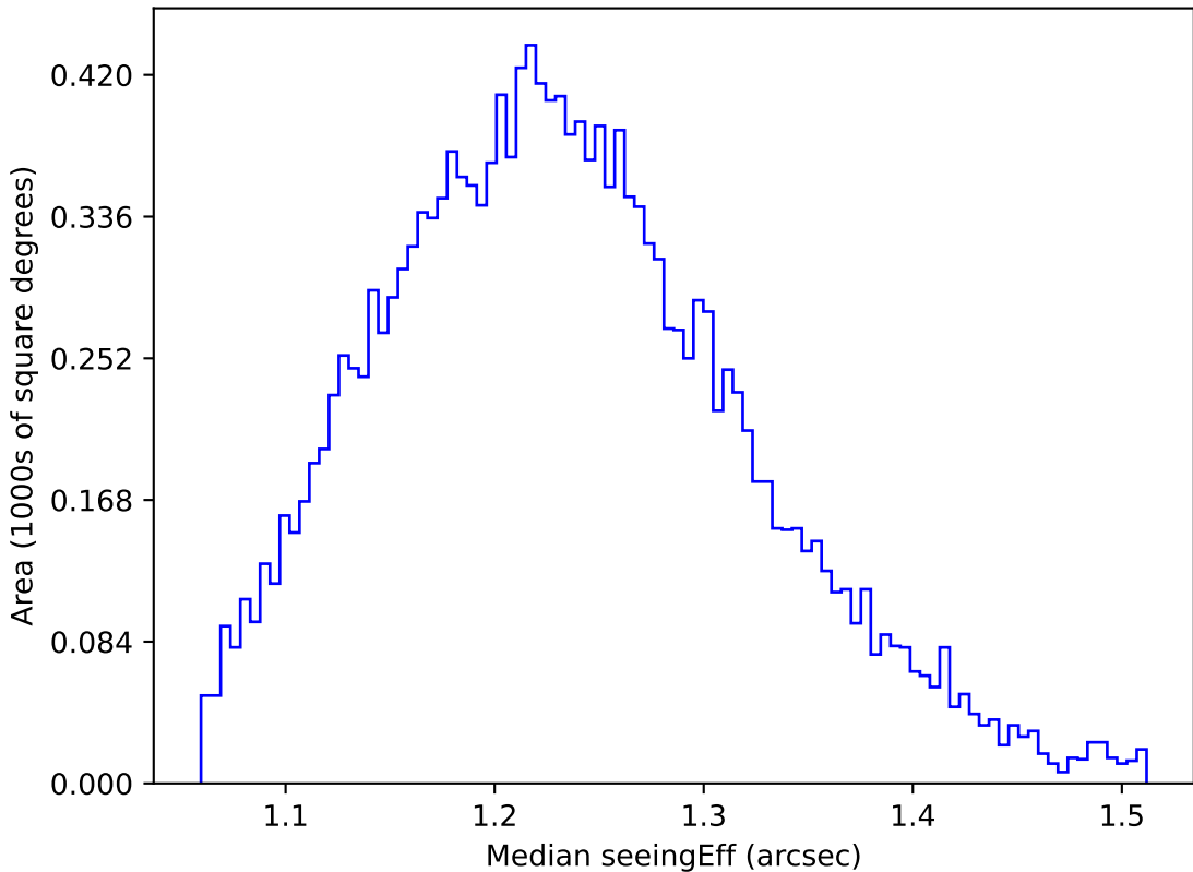
too_elab_r32_d3_giz_v3.4_10yrs WFD u band: Median seeingEff
