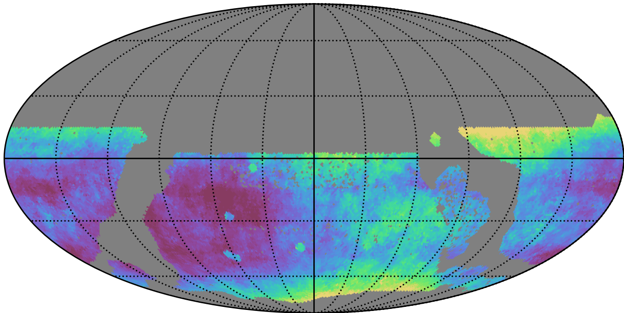
too_elab_r32_d3_giz_v3.4_10yrs WFD r band: Median seeingEff
