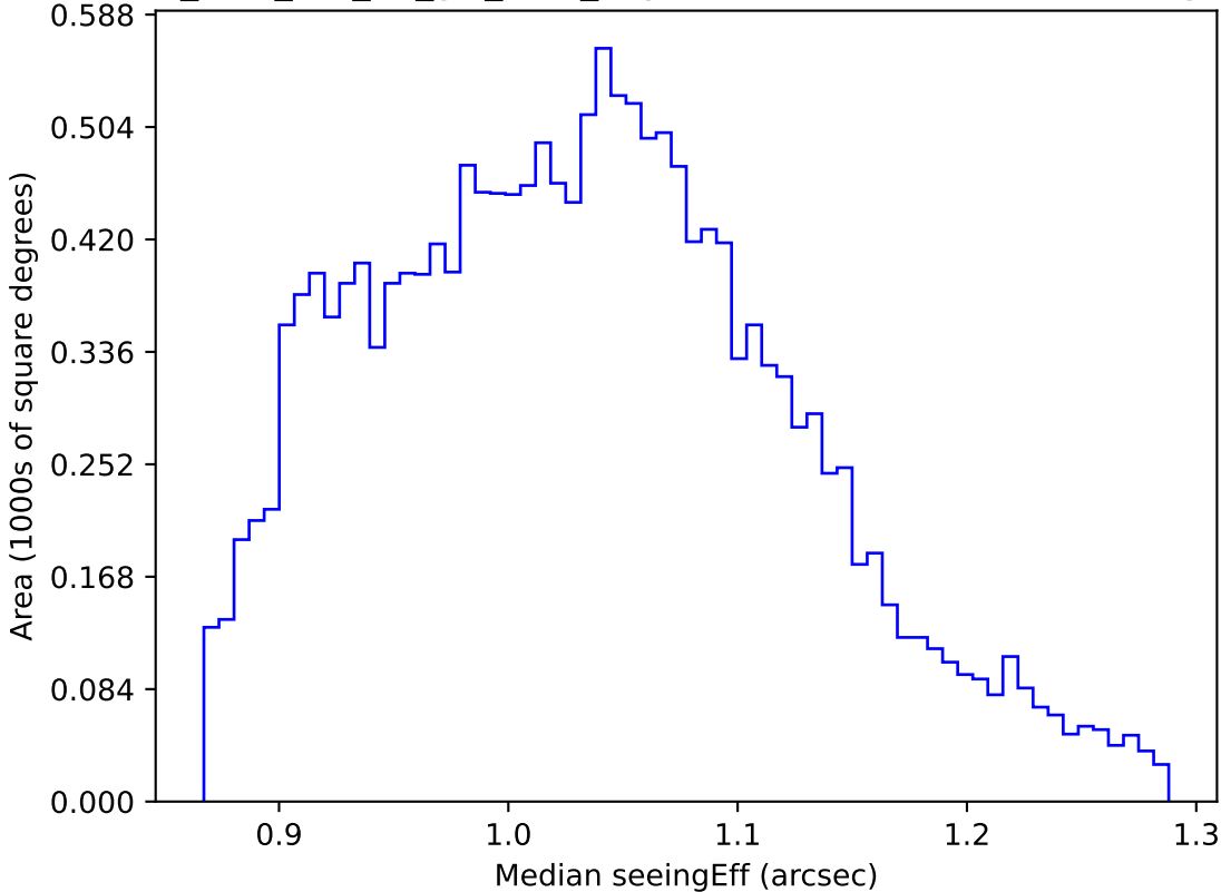
too_elab_r32_d3_giz_v3.4_10yrs WFD r band: Median seeingEff
