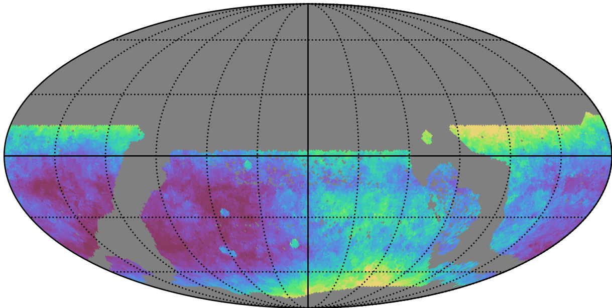
too_elab_r32_d3_giz_v3.4_10yrs WFD i band: Median seeingEff
