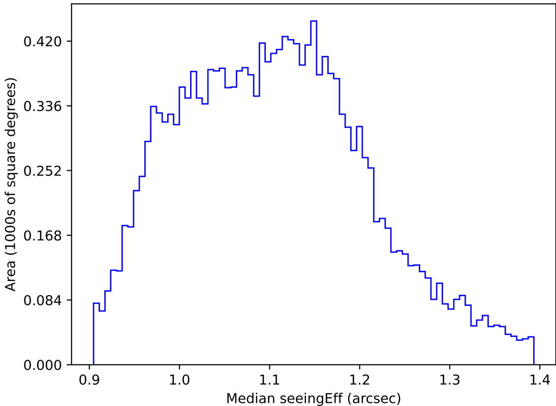
too_elab_r32_d3_giz_v3.4_10yrs WFD g band: Median seeingEff
