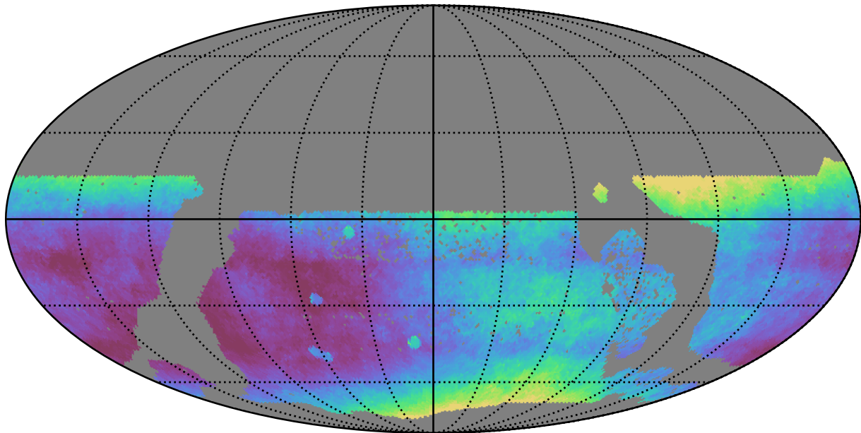
too_elab_r32_d3_giz_v3.4_10yrs WFD all bands: Median seeingEff
