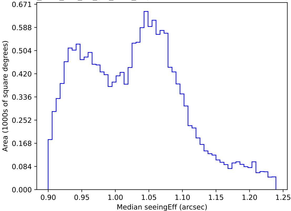
too_elab_r32_d3_giz_v3.4_10yrs WFD all bands: Median seeingEff
