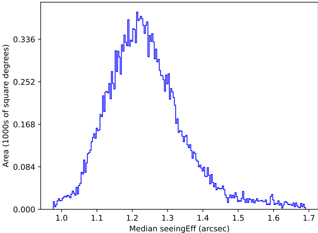
too_elab_r32_d3_giz_v3.4_10yrs All sky u band: Median seeingEff
