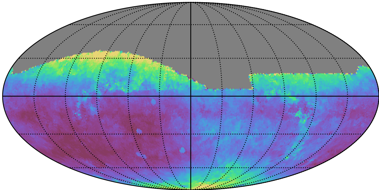
too_elab_r32_d3_giz_v3.4_10yrs All sky i band: Median seeingEff
