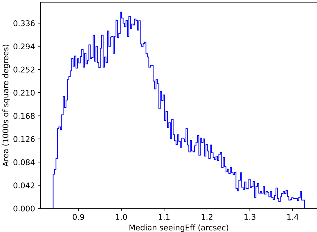
too_elab_r32_d3_giz_v3.4_10yrs All sky i band: Median seeingEff
