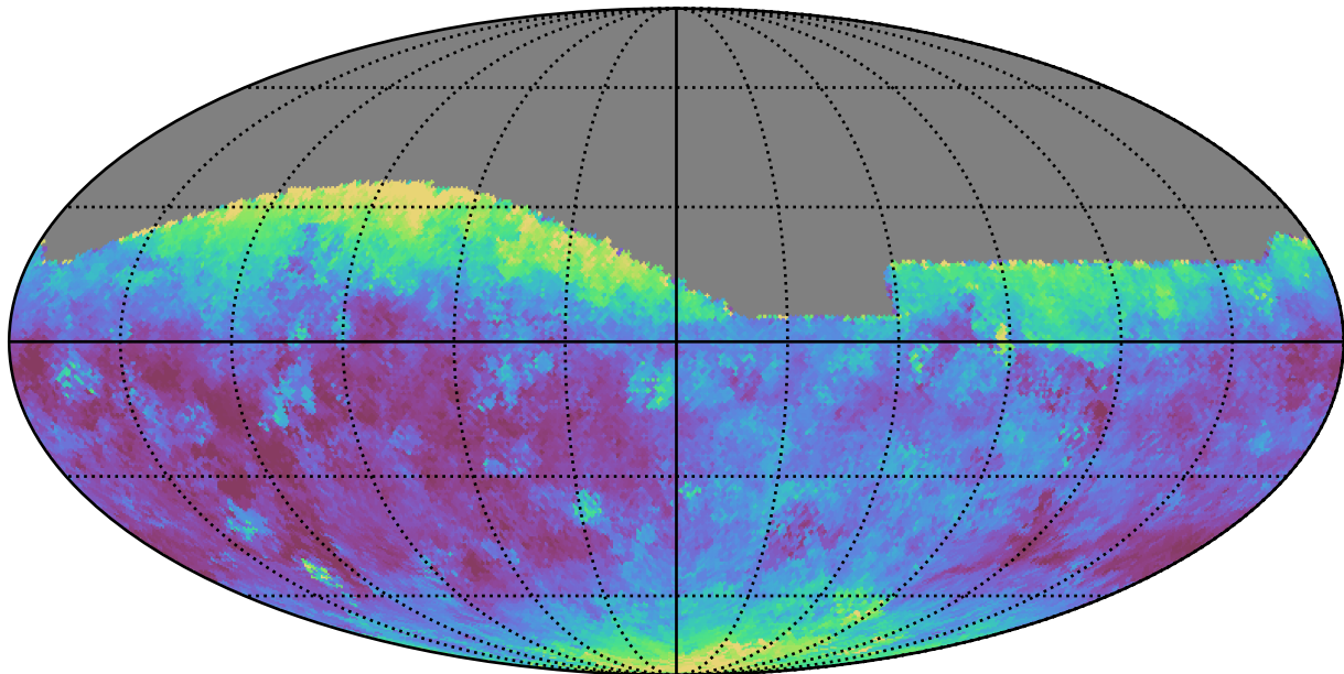
too_elab_r32_d3_giz_v3.4_10yrs All sky g band: Median seeingEff
