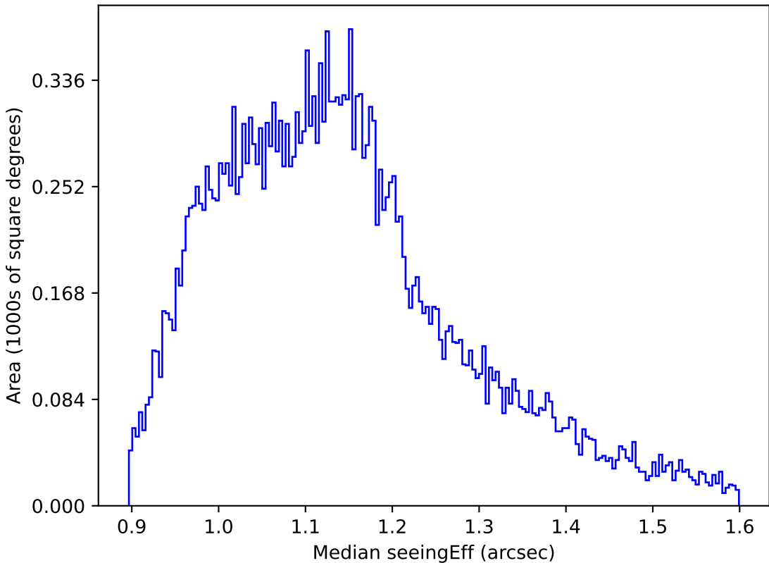
too_elab_r32_d3_giz_v3.4_10yrs All sky g band: Median seeingEff
