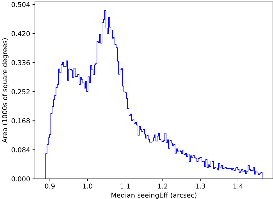
too_elab_r32_d3_giz_v3.4_10yrs All sky all bands: Median seeingEff
