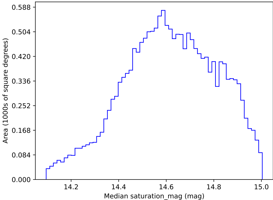
too_elab_r32_d3_giz_v3.4_10yrs WFD r band: Median saturation_mag
