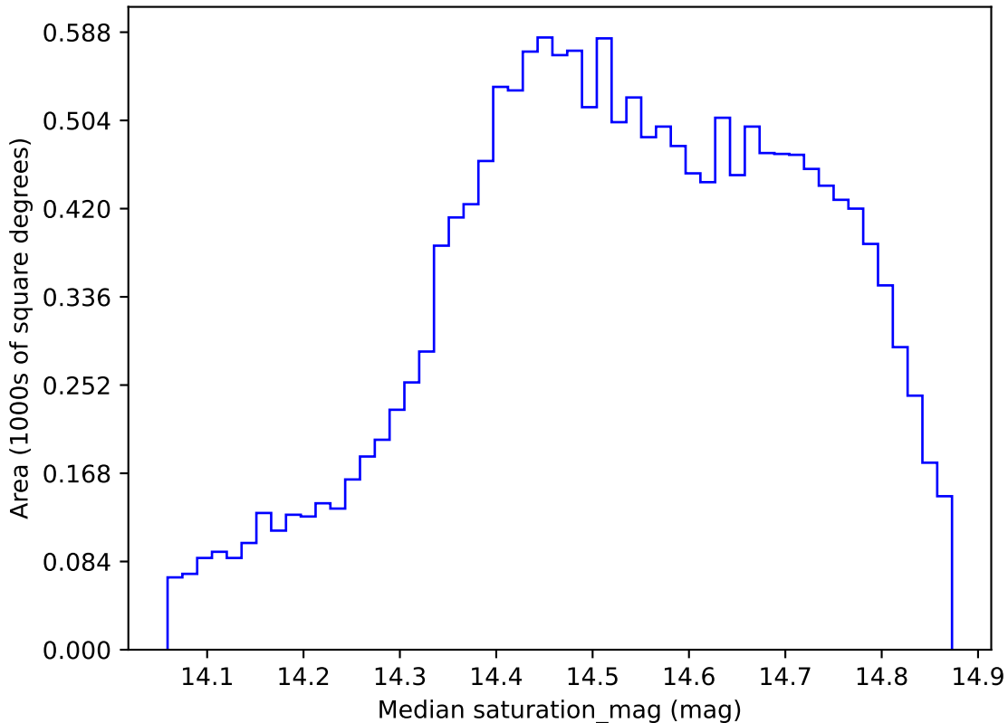
too_elab_r32_d3_giz_v3.4_10yrs WFD i band: Median saturation_mag
