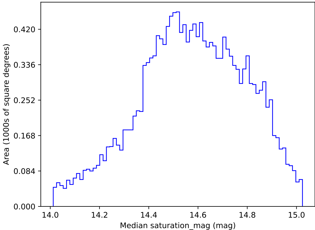
too_elab_r32_d3_giz_v3.4_10yrs WFD g band: Median saturation_mag
