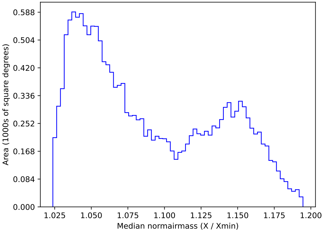
too_elab_r32_d3_giz_v3.4_10yrs WFD z band: Median normairmass
