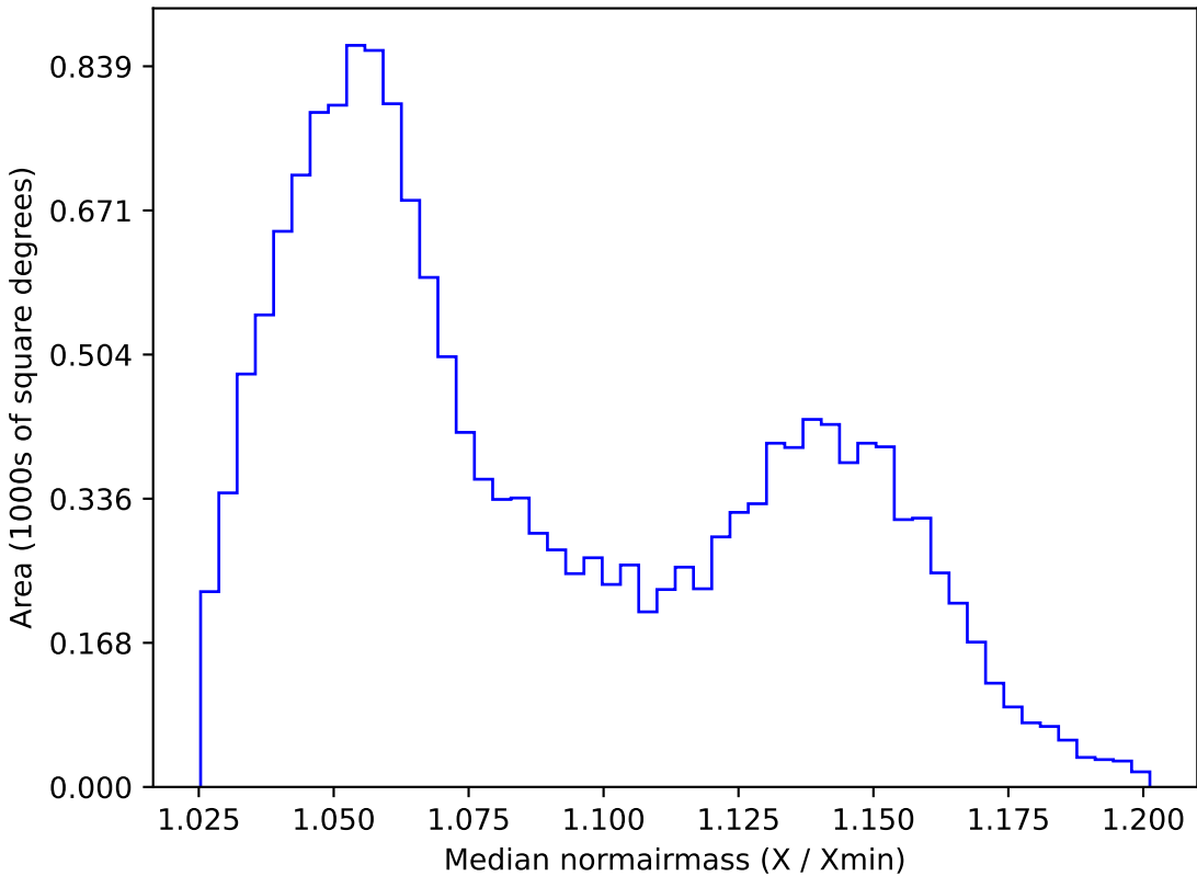
too_elab_r32_d3_giz_v3.4_10yrs WFD y band: Median normairmass
