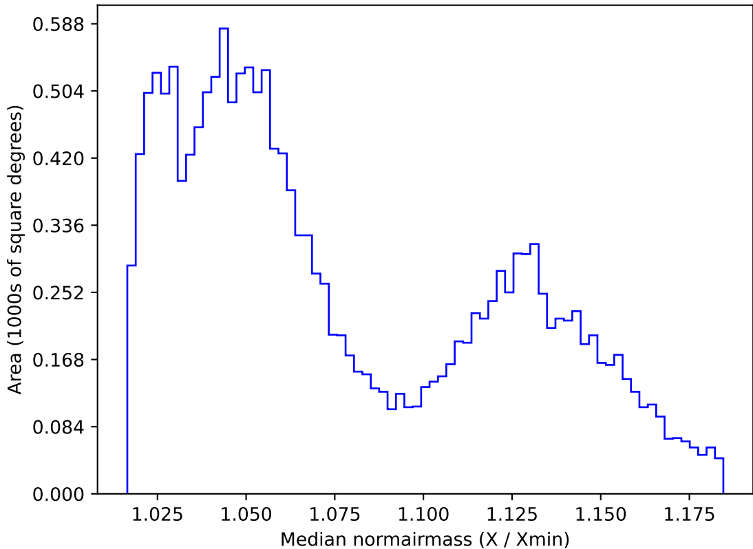
too_elab_r32_d3_giz_v3.4_10yrs WFD r band: Median normairmass
