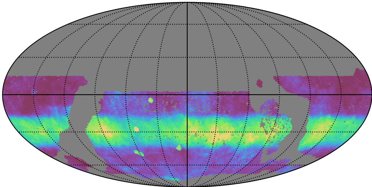
too_elab_r32_d3_giz_v3.4_10yrs WFD i band: Median normairmass
