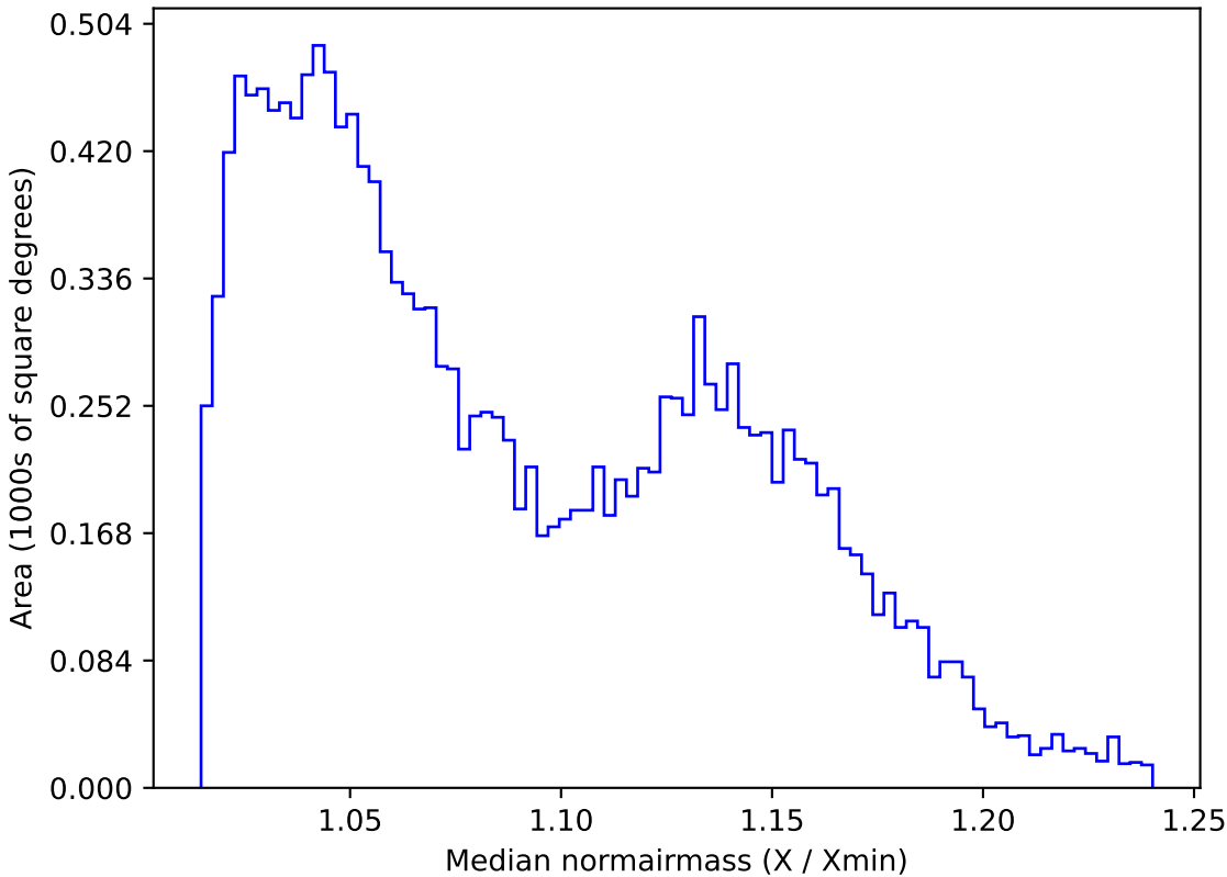
too_elab_r32_d3_giz_v3.4_10yrs WFD g band: Median normairmass
