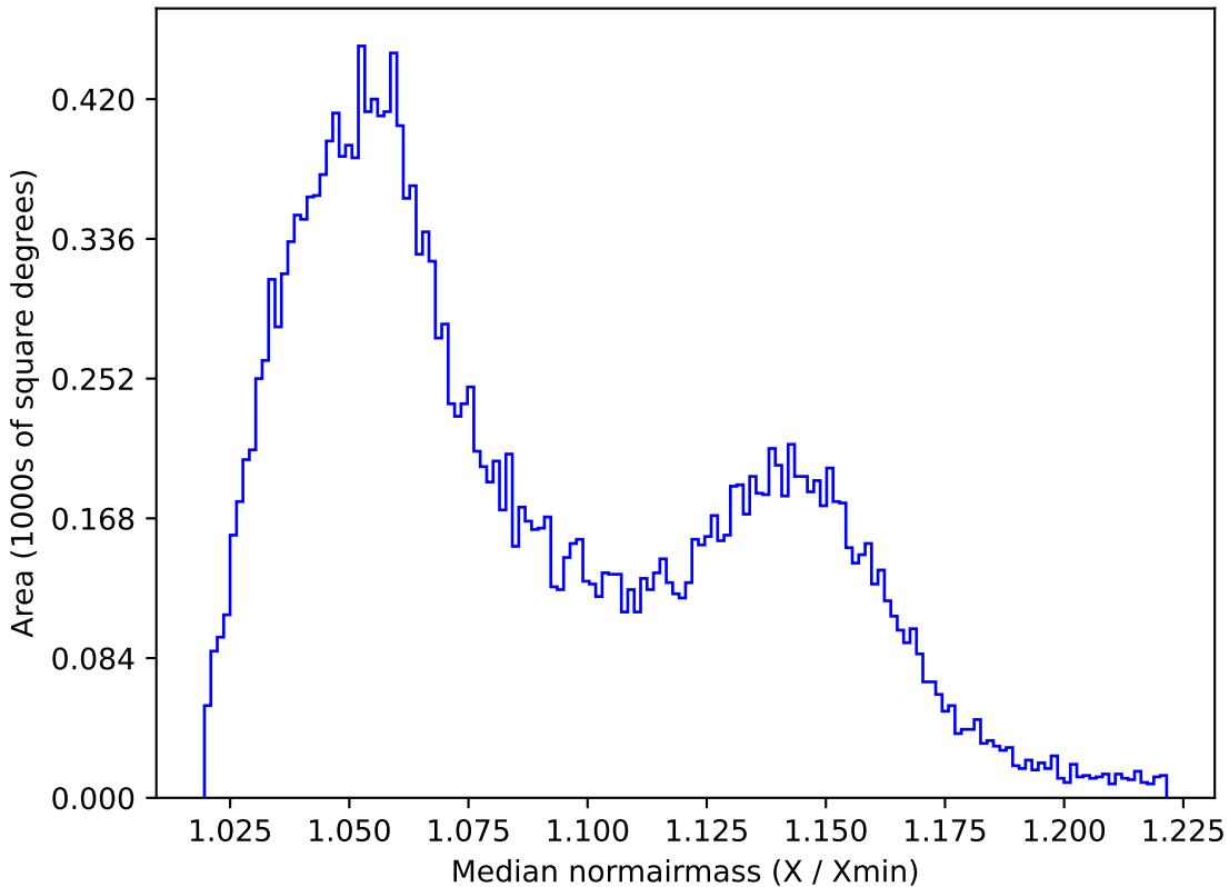
too_elab_r32_d3_giz_v3.4_10yrs All sky y band: Median normairmass
